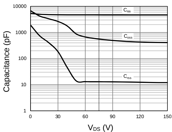
Figure 11. Capacitance
