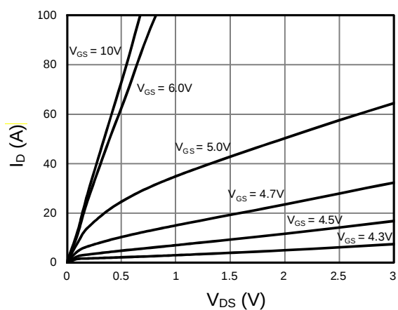
Figure 3. Output characteristics
