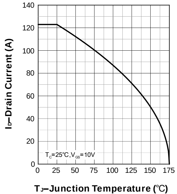
Current Capability
