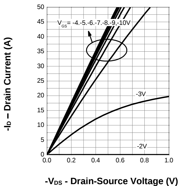
Output Characteristics
