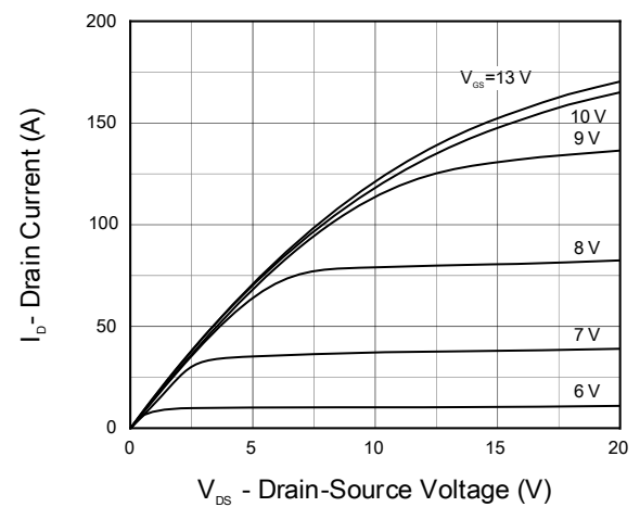
Fig 6. Output Characteristics T_J = 150^\circ\text{C}
