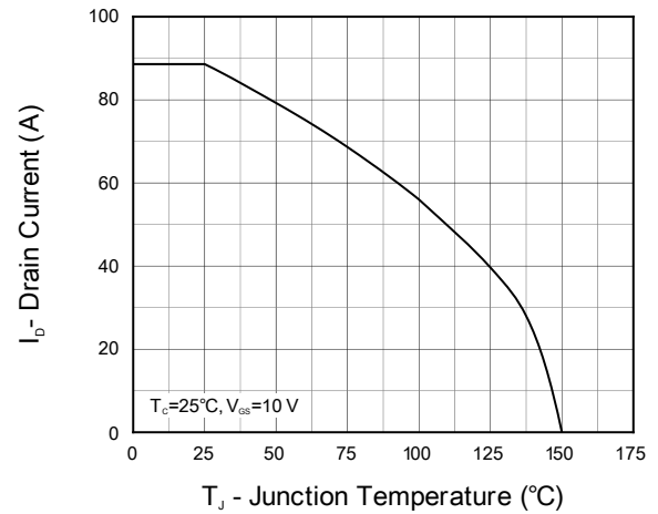
Fig 2. Current Capability
