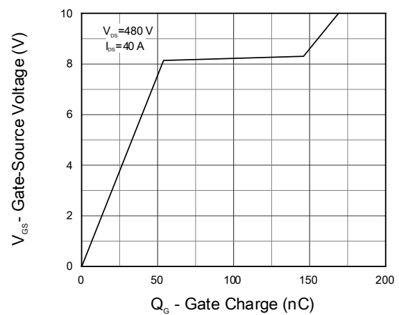
Fig 12. Gate Charge
