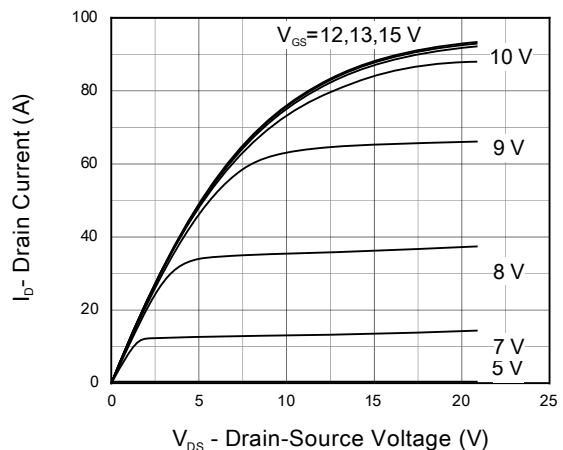
Fig 5. Output Characteristics T_J=25^\circ\text{C}
