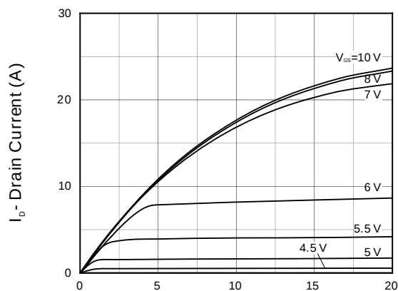
Fig 6. Output Characteristics T_J=150^\circ\text{C}
