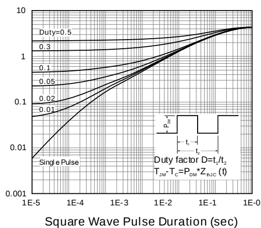
Fig 4. Transient Thermal Impedance
