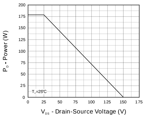
Fig 1. Power Capability
