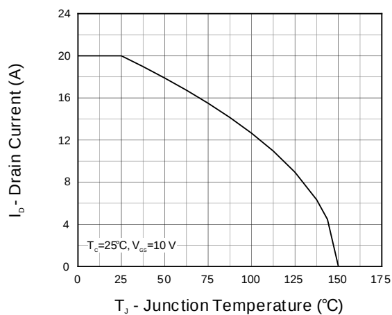
Fig 2. Current Capability
