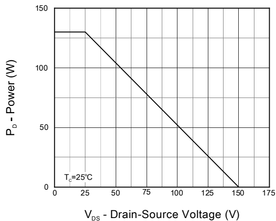
Fig 1. Power Characteristics
