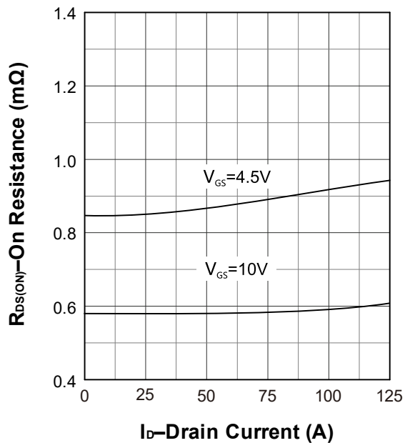
On Resistance
