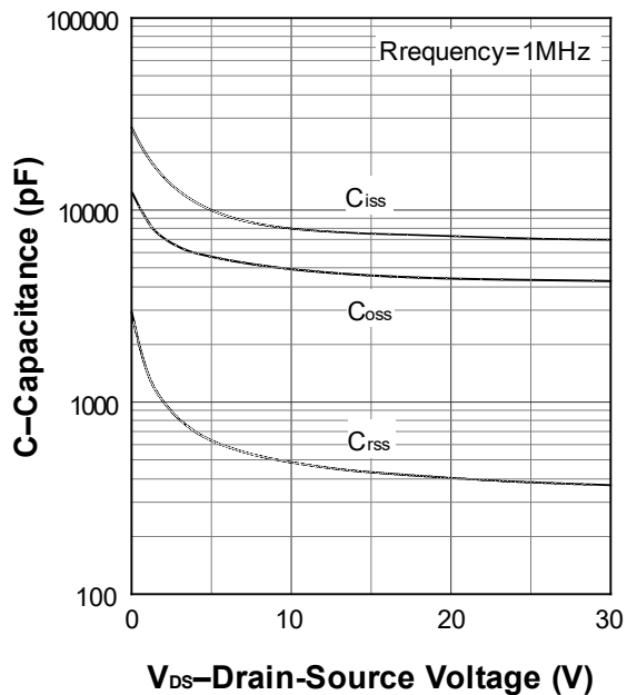
Capacitance
