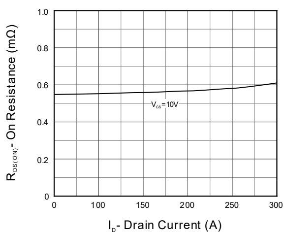
Figure 6. On Resistance
