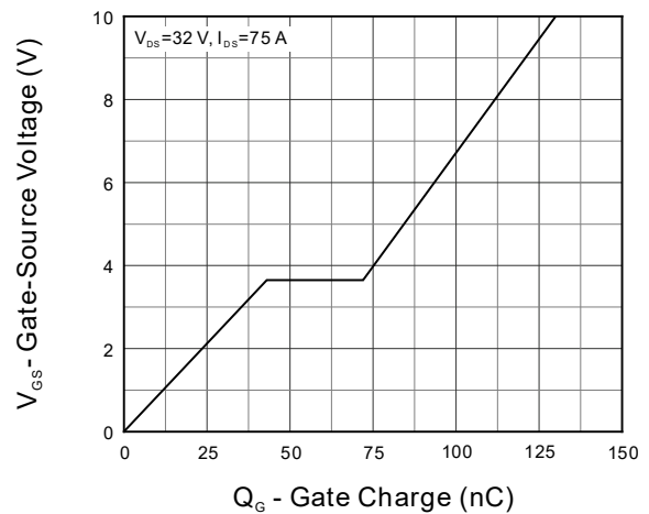
Fig 12. Gate Charge
