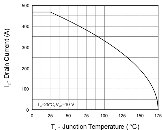
Fig 2. Current Capability
