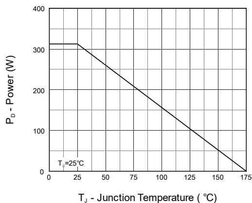
Fig 1. Power Capability
