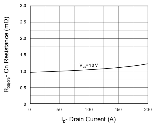
Fig 6. On Resistance
