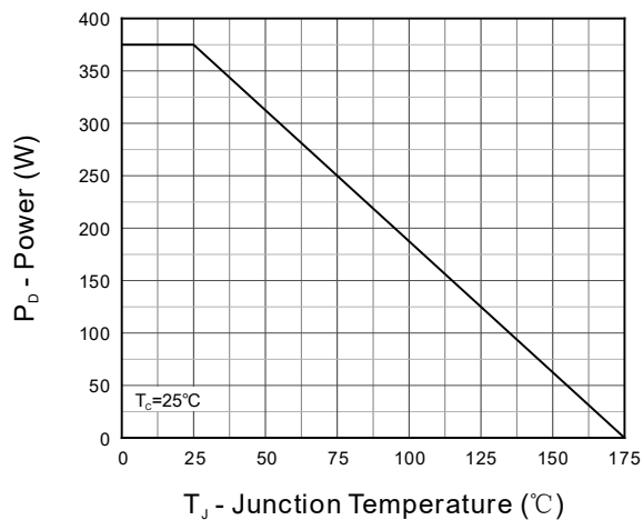
Figure 1. Power Capability
