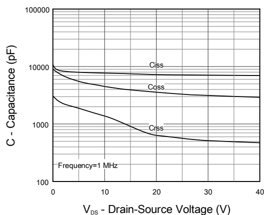
Figure 11. Capacitance
