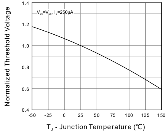
Figure 8. Normalized V_{GS(th)}
