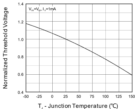
Figure 8. Normalized V_{GS(th)}
