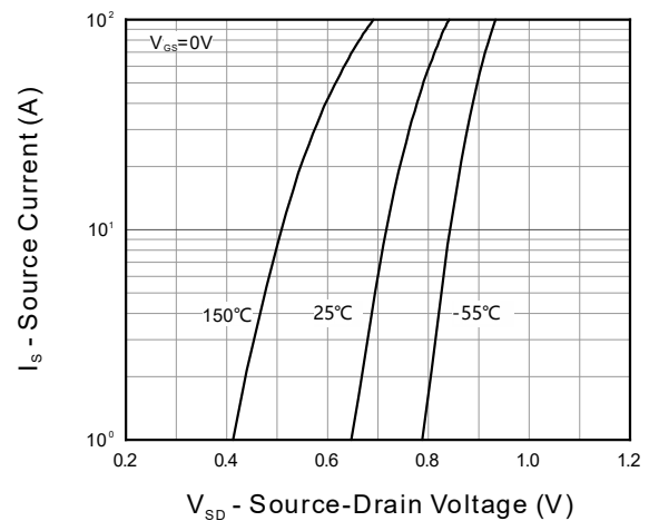
Figure 10. Diode Forward Current
