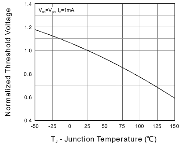
Figure 8. Normalized V_{GS(th)}
