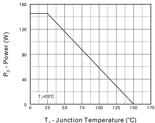
Figure 1. Power Capability
