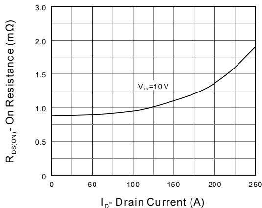
Figure 6. On Resistance
