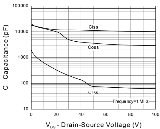
Figure 11. Capacitance
