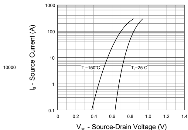
Figure 10. Diode Forward Current
