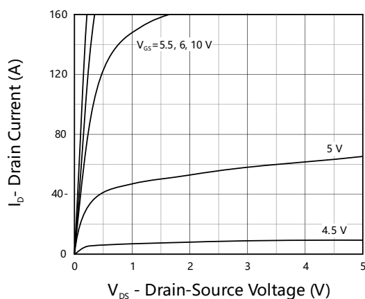
Fig 5. Output Characteristics
