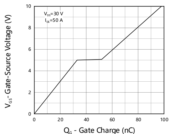
Fig 12. Gate Charge
