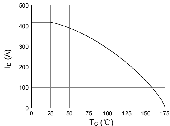
Figure 2. Current Capability
