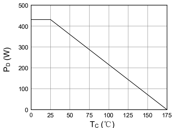
Figure 1. Power Capability
