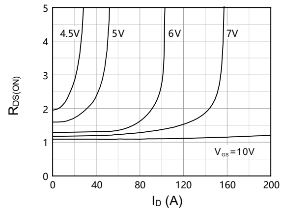
Figure 6. On-resistance vs I_D
