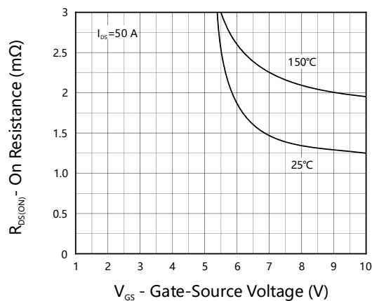
Fig 7. Transfer Characteristics
