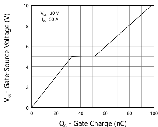
Fig 12. Gate Charge
