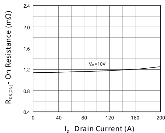
Fig 6. On Resistance
