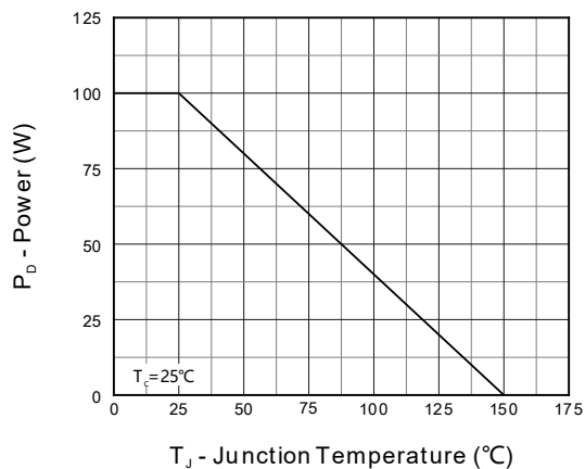
Figure 1. Power Capability
