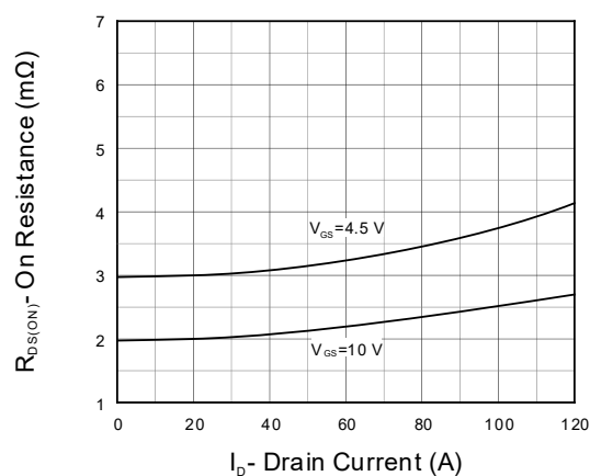
Figure 6. On Resistance
