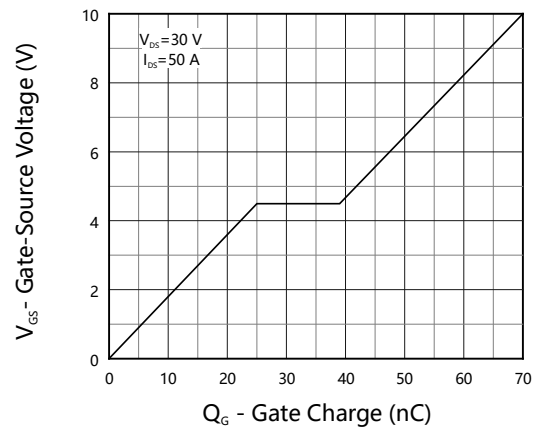
Fig 12. Gate Charge
