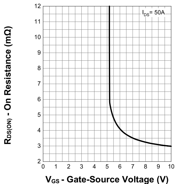
Transfer Characteristics
