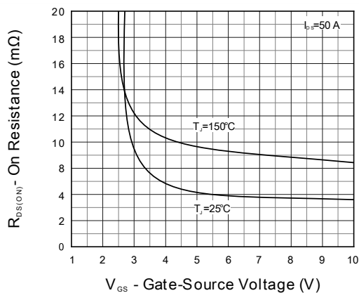
Figure 7. Transfer Characteristics
