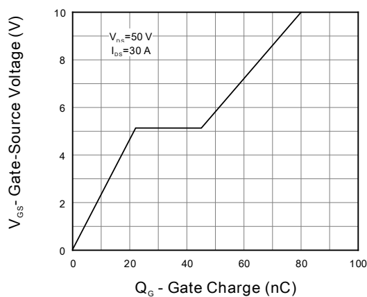
Figure 12. Gate Charge
