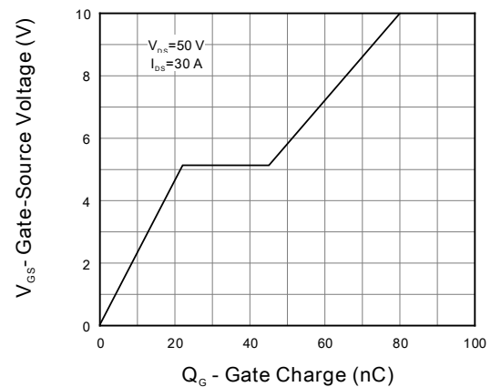
Figure 12. Gate Charge
