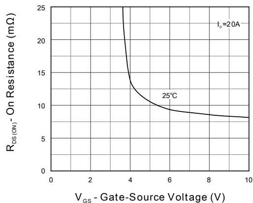
Figure 7. Drain-Source on resistance
