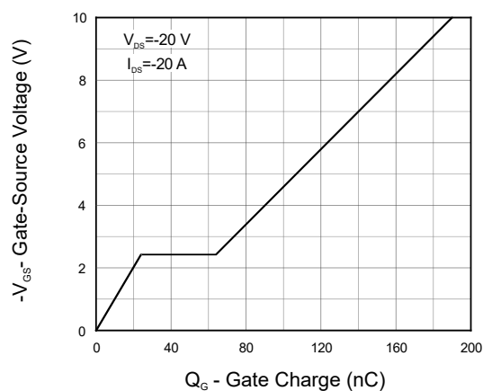
Figure 12. Gate Charge
