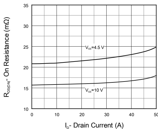
Figure 6. On Resistance
