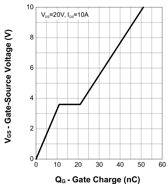
Gate Charge
