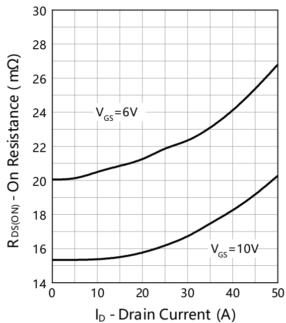
On Resistance
