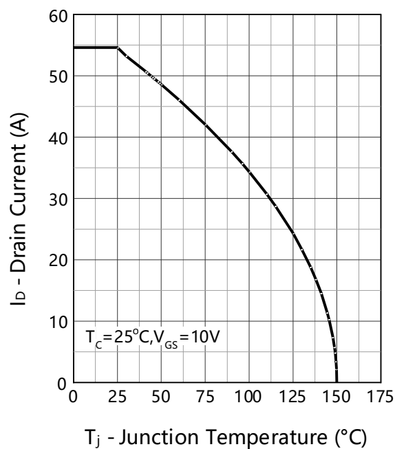
Current Capability
