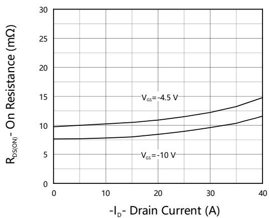
Figure 6. On Resistance
