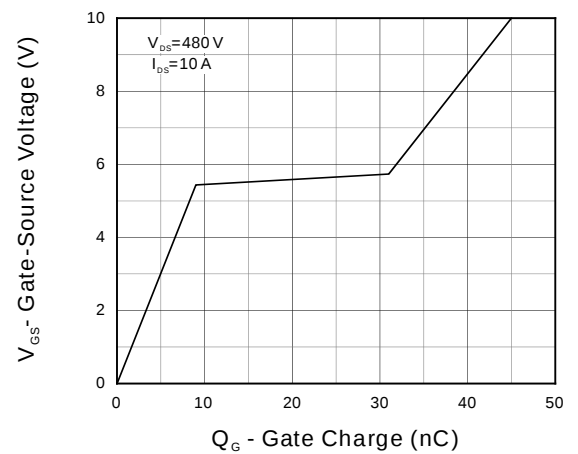
Fig 12. Gate Charge
