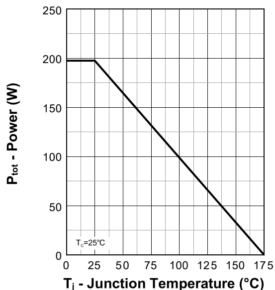
Power Capability
