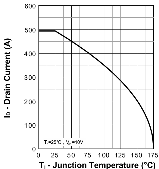
Current Capability
