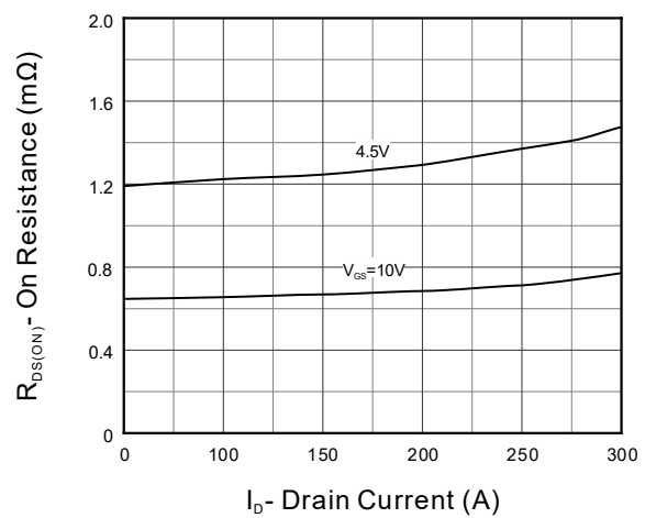
Figure 6. On Resistance
