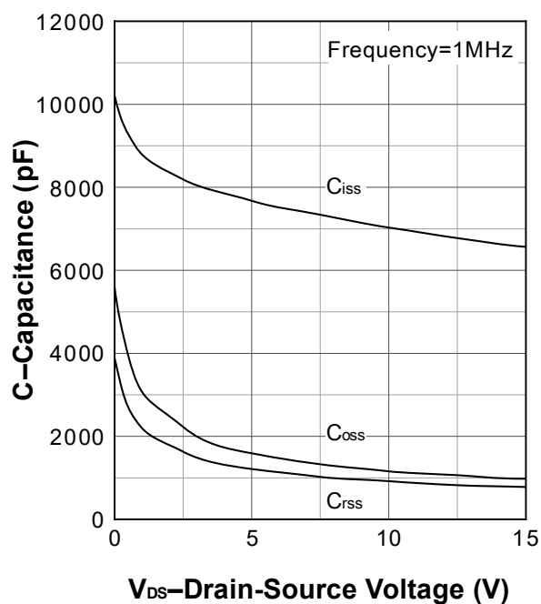
Capacitance
