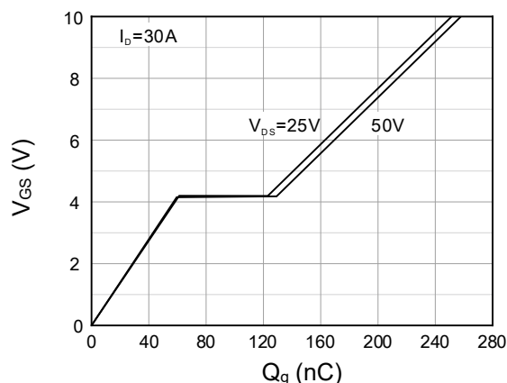
Figure 12. Gate charge
