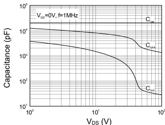
Figure 11. Capacitance
