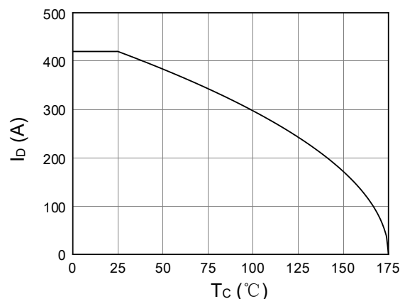
Figure 2. Current Capability
