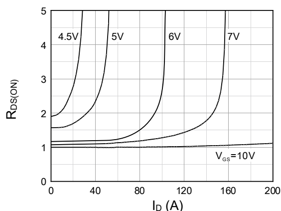
Figure 6. On-resistance vs I_D
