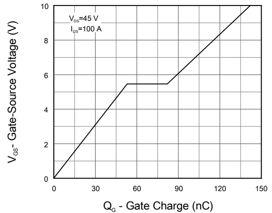
Figure 12. Gate Charge
