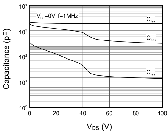
Figure 11. Capacitance
