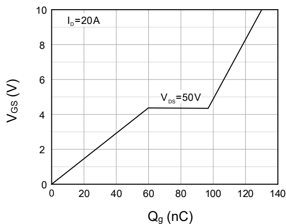
Figure 12. Gate charge
