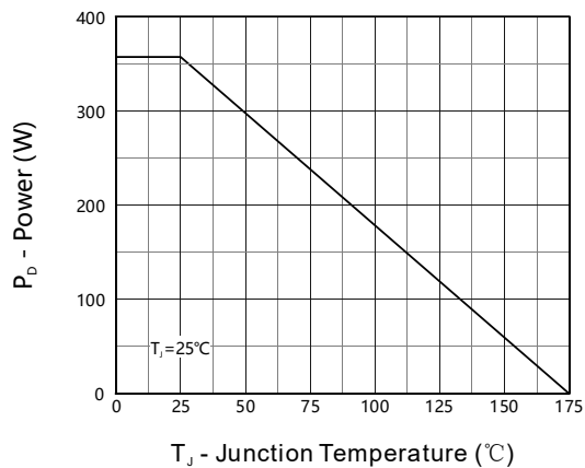
Fig 1. Power Capability
