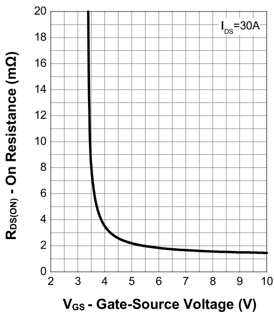
Transfer Characteristics
