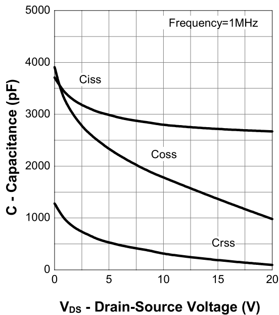
Capacitance
