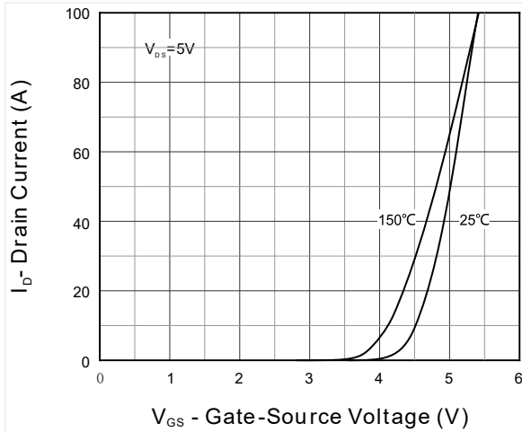
Figure 7. Transfer Characteristics
