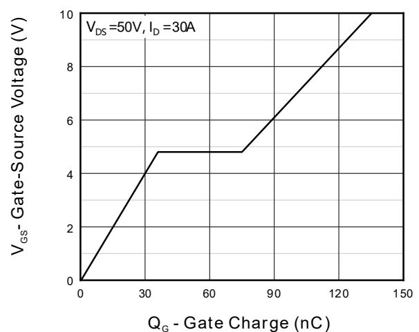
Figure 12. Gate Charge
