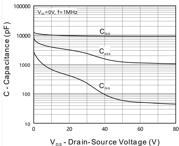
Figure 11. Capacitance
