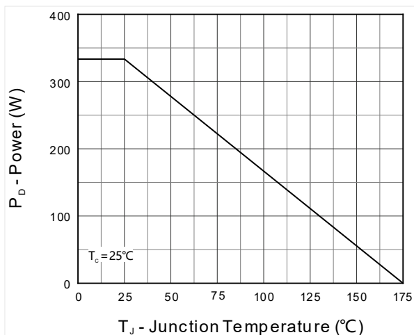
Figure 1. Power Capability
