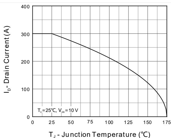
Figure 2. Current Capability
