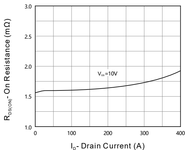
Figure 6. On Resistance
