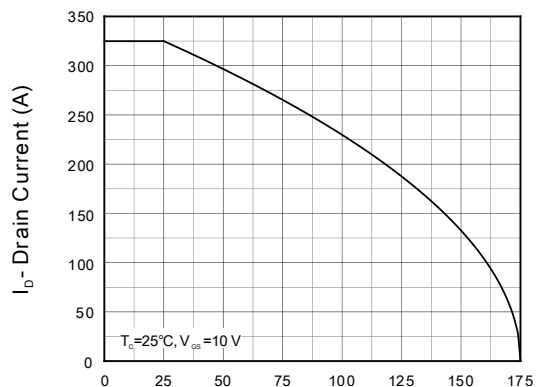
Figure 2. Current Capability
